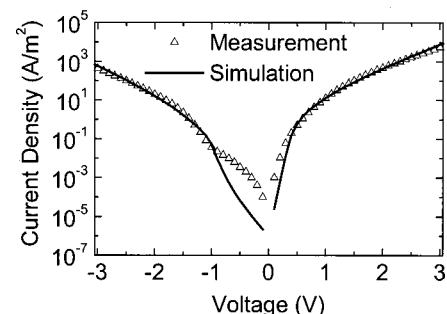
FIG. 1. Comparison between the J-V curves measured and simulated in an ultrathin oxide n -MOSFETs. A perfect agreement is observed except at low negative voltages.
