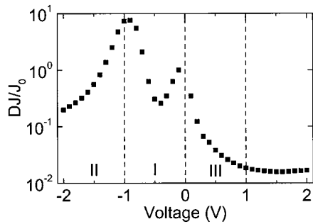
FIG. 2. Relative increase of the current density, DJ/J_0 , after a high field stress as a function of the gate voltage in ultrathin oxide n -MOSFETs. At voltages lower than about 1 V, DJ/J_0 is higher and voltage dependent.
